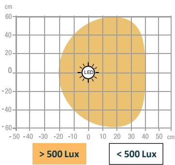
Measurement in lux on the work surface from a top view at 40 cm :
