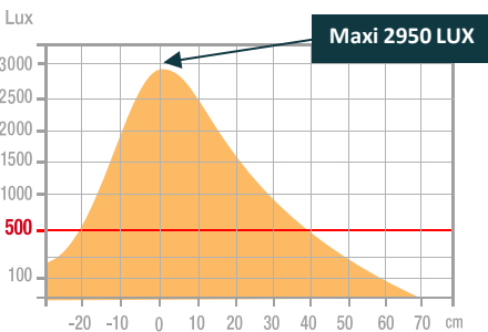
Measurement in lux on the work surface from a side view at 40 cm :
